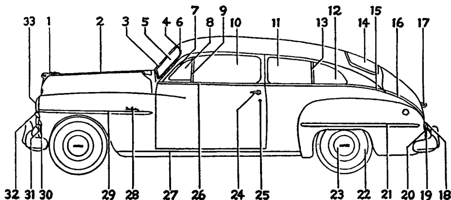
Fig. 3—Moldings, Wheels and Glass, 2-door
