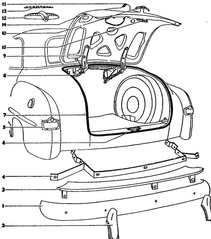
Fig. 14—Rear Luggage Compartment & Rear Bumper
