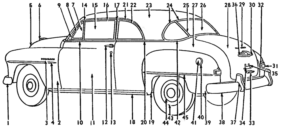
Fig. 8—Body Moldings, Wheels and Glass
