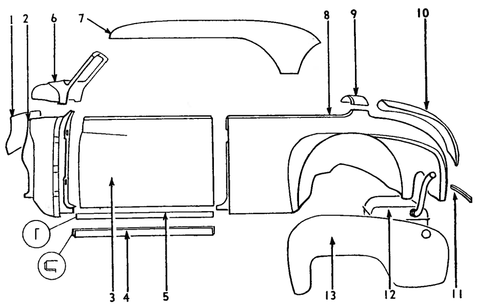
Fig. 10—Body Sheet Metal and Fuel Tank
