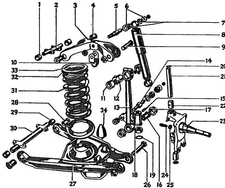
Fig. 16—Front Suspension
