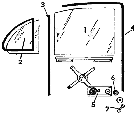
Fig. 11—Rear Quarter Window, Tudor Sedan
