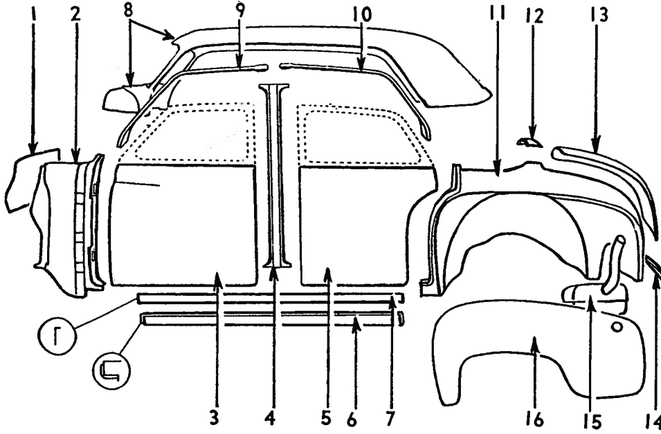
Fig. 4—Body Sheet Metal and Fuel Tank, 4-door
