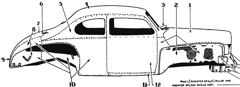
Body Sheet Metal
