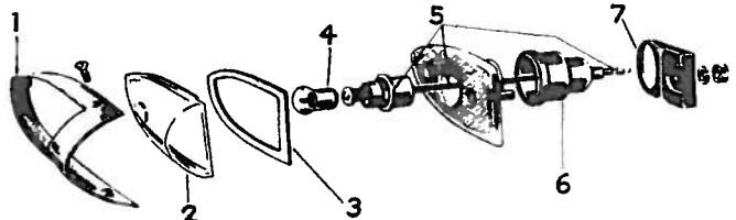
PARKING LAMP ALL MODELS
