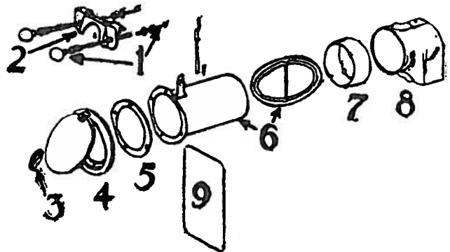
VENTILATING SYSTEM ALL MODELS
