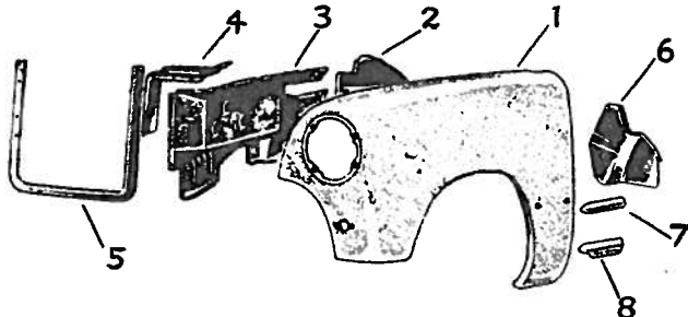
FRONT FENDER ALL MODELS
