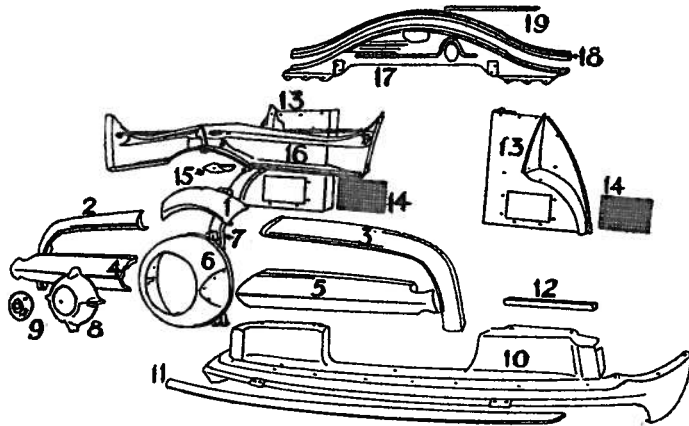
GRILLE ALL MODELS
