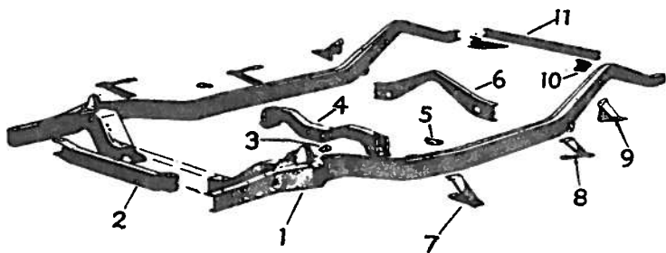
FRAME EXCEPT BODY TYPE 79
