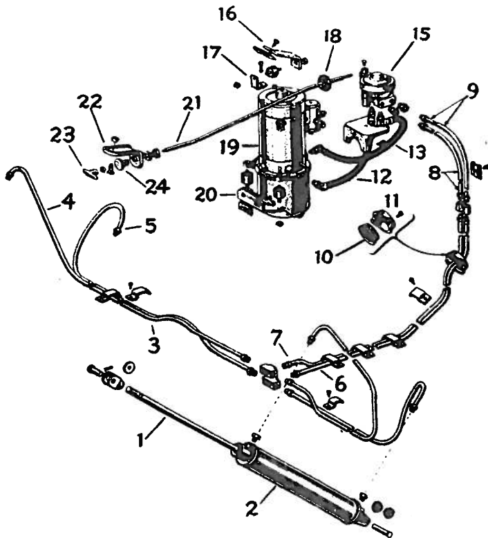
CONVERTIBLE TOP LIFTING MECHANISM BODY TYPE 76
