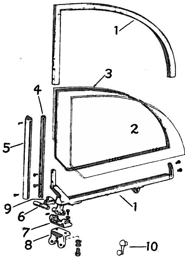
QUARTER WINDOW BODY TYPE 76—CONVERTIBLE
