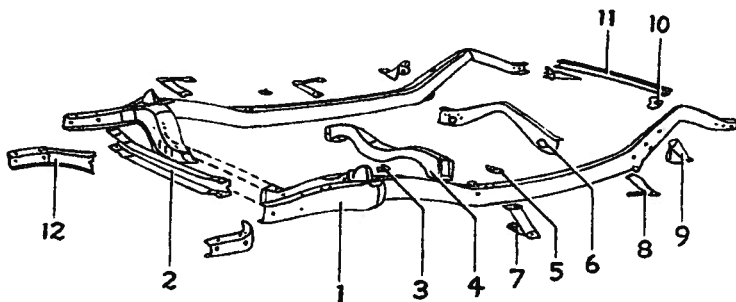
Frame Assembly. All Except Body Type 79
