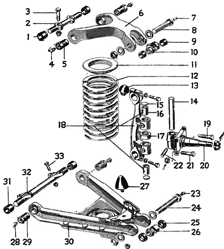
Front Suspension
