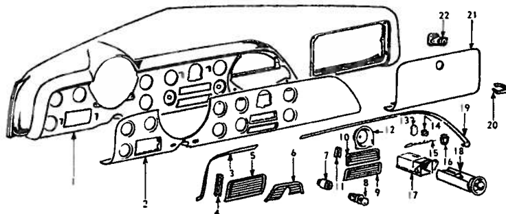
Fig. 2—Instrument Panel
