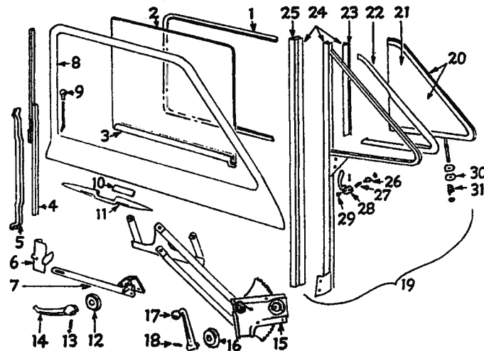
Fig. 6—Front Doors—Typical of Body Types 70, 72, 73
