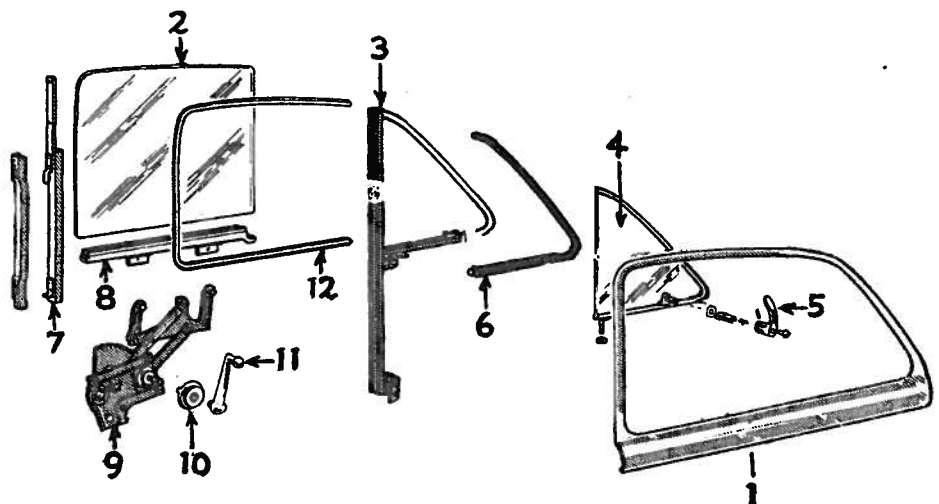
Fig. 8—Quarter Window—Body Type 70
