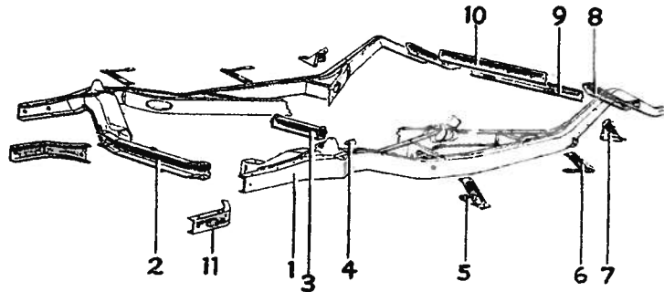
Frame—Body Style 79
