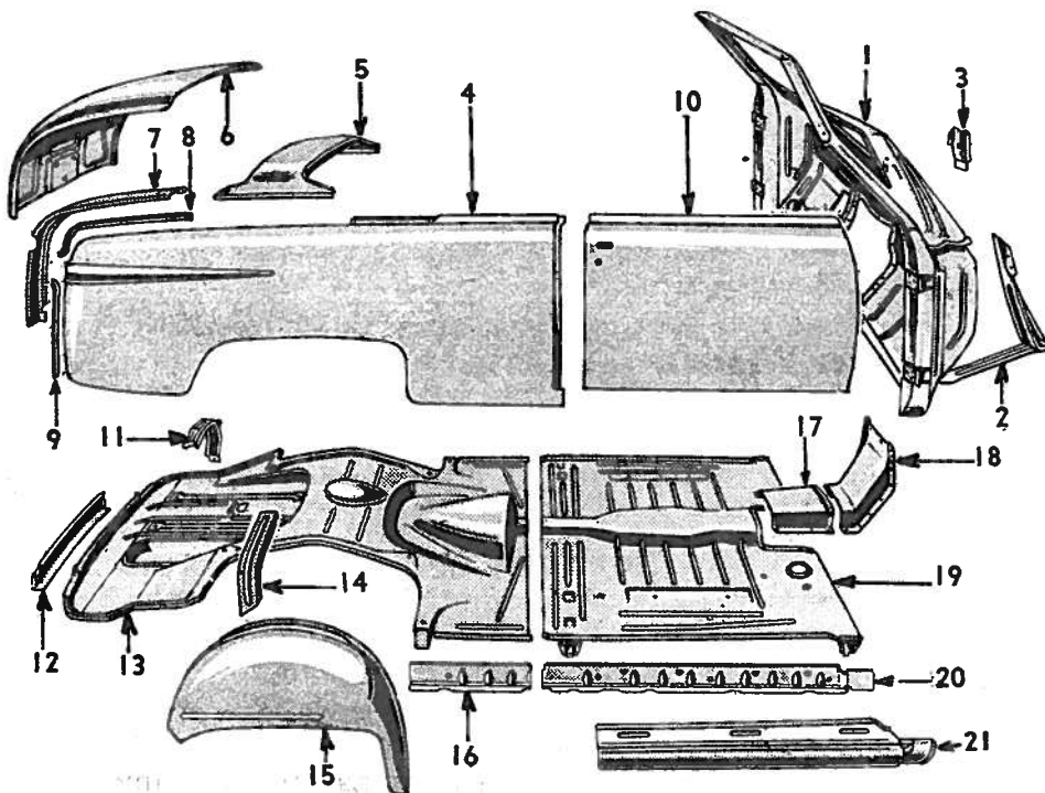
Fig. 14—Sheet Metal—Convertible
