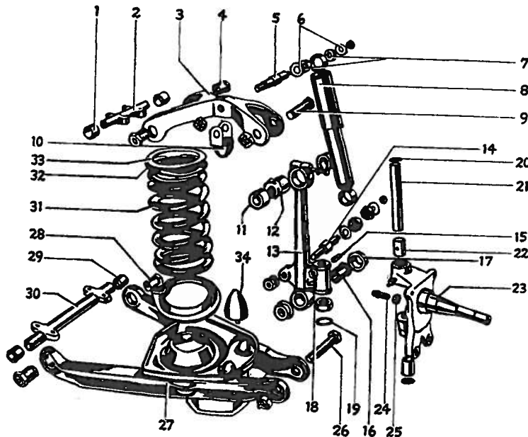
Fig. 15—Front Suspension Parts
