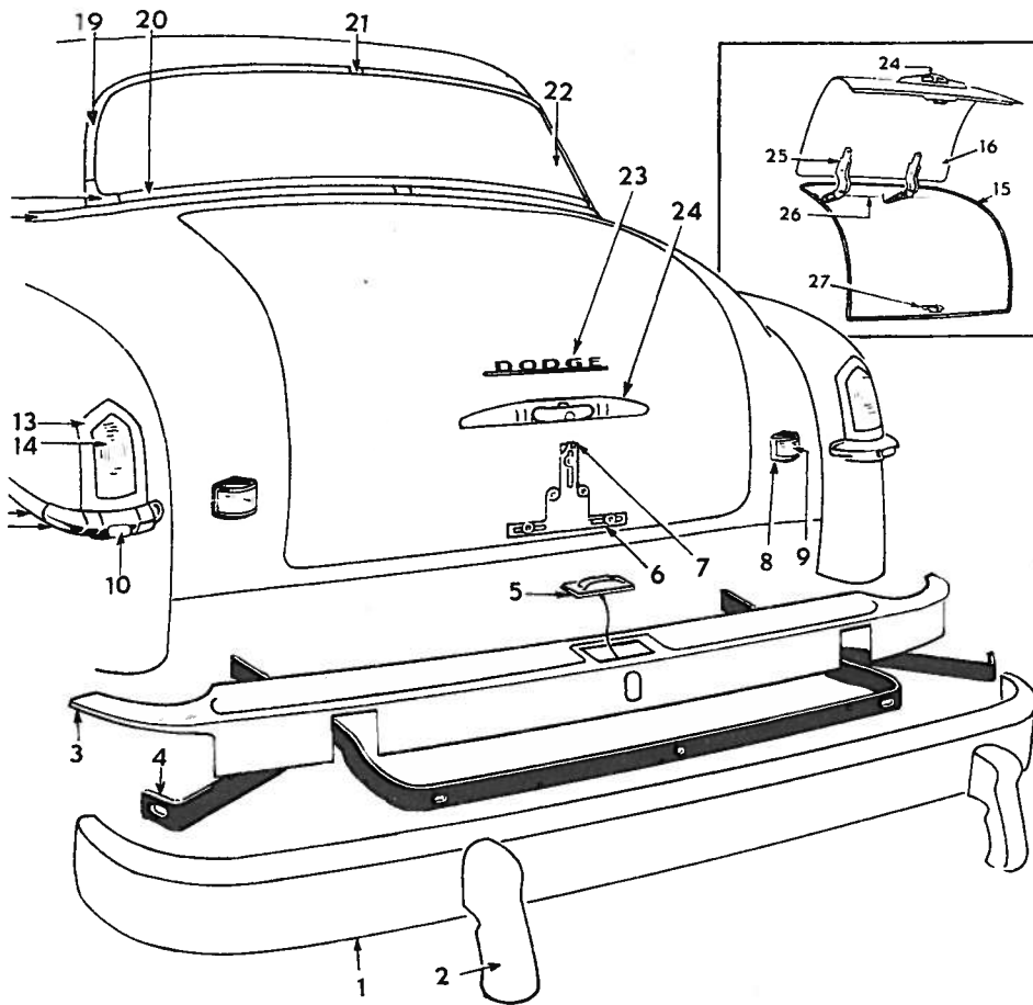
Fig. 14—Rear End Sheet Metal (1950 Illustrated)
