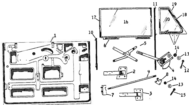
Fig. 11—Door Assembly, Convertible, Coupe and Roadster
