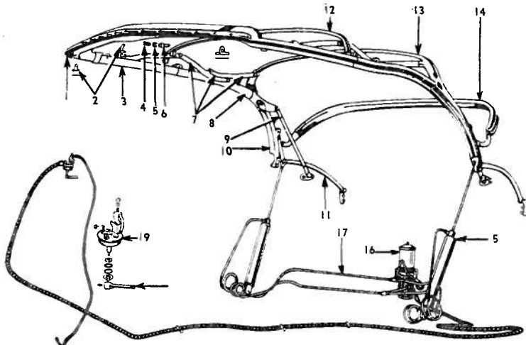
Fig. 12—Folding Top Assembly
