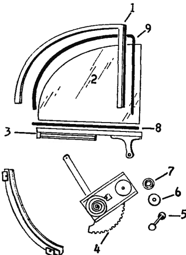
Fig. 10—Quarter Window
