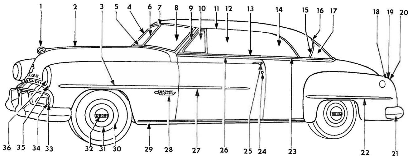
Fig. 8—Body Moldings
