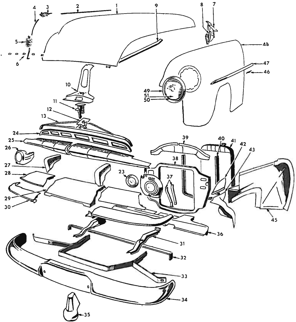
Fig. 1—Front End of Car—1951-52—Illustrated Typical of 1953
