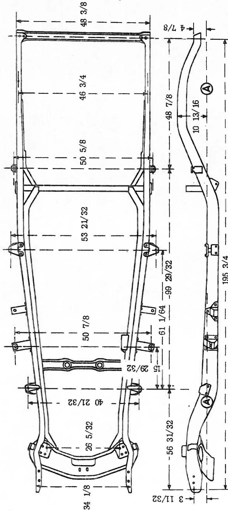
Frame Alignment (Dimensions given in inches) A—Top Line of Frame
