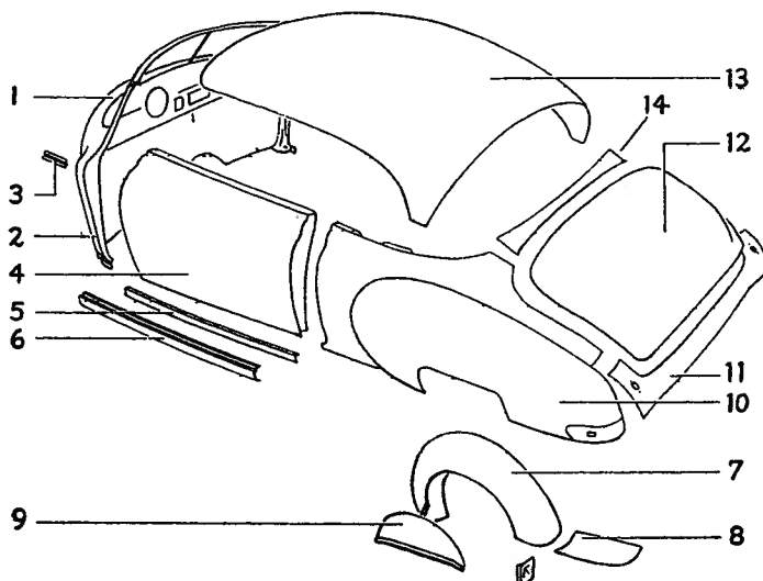
Fig. 11—Body Sheet Metal and Fuel Tank
