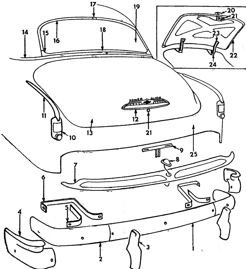
Fig. 17—Rear of car sheet metal
