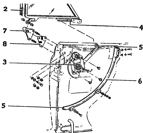
Fig. 12—Rear Quarter Window, Bel Air & Cabriolet
