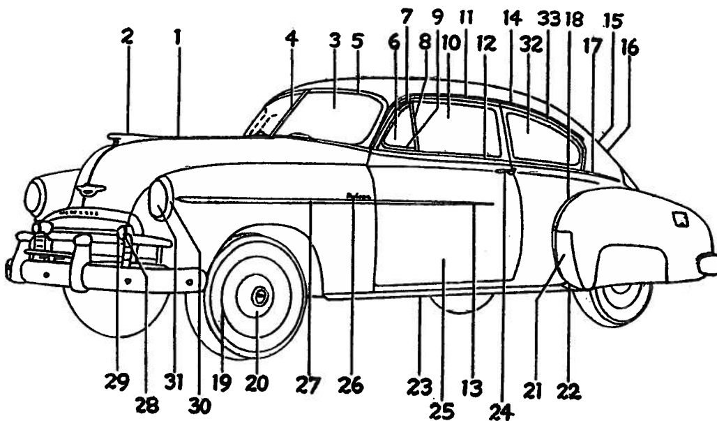
Fig. 5—Body Moldings, Wheels and Glass—2-Door Sedans and Coupes
