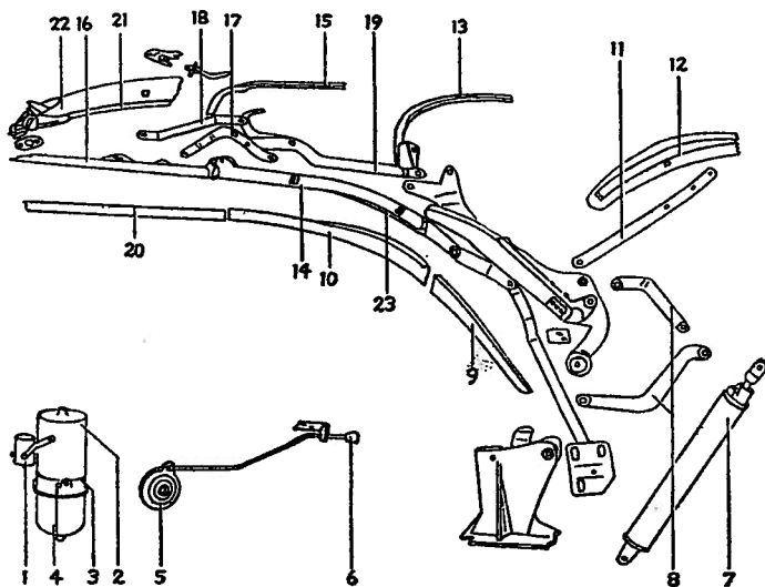
Fig. 13—Hydro-Electric Power Top (Left Side Part Numbers Shown) Cabriolet
