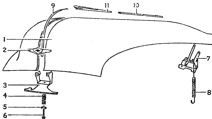
Fig. 2—Hood Assembly—Typical of all models—1949 to 1953
