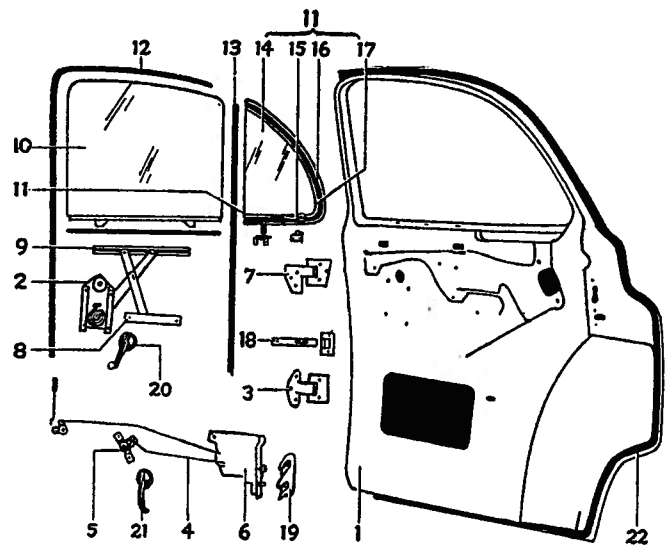
Fig. 16—Rear Door (Left Side Part Numbers Shown) 4-Door Sedans and Station Wagons
