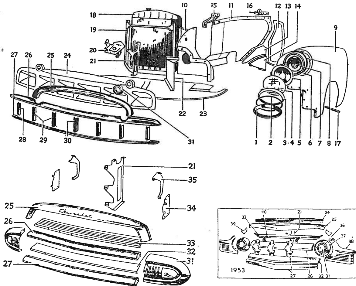
Fig. 1—Front Fender, Grilles, Lamps & Radiator; Typical of all 1949-53 models
