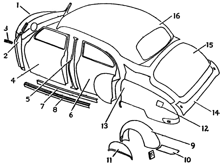
Fig. 6—Body Sheet Metal and Fuel Tank
