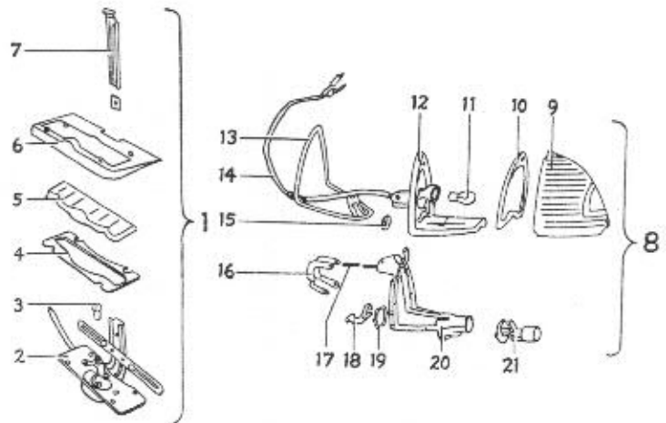
REAR & TAIL LAMPS ALL MODELS
