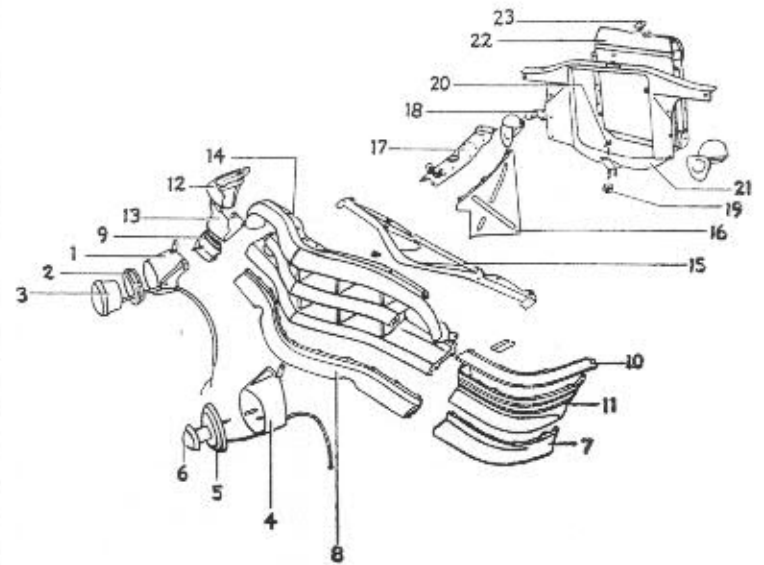
RADIATOR, GRILLE & SHIELD ALL MODELS
