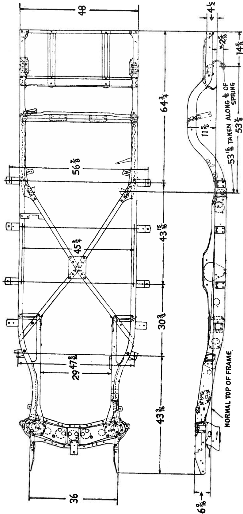
Frame Dimensions—Series 2201, 2211
