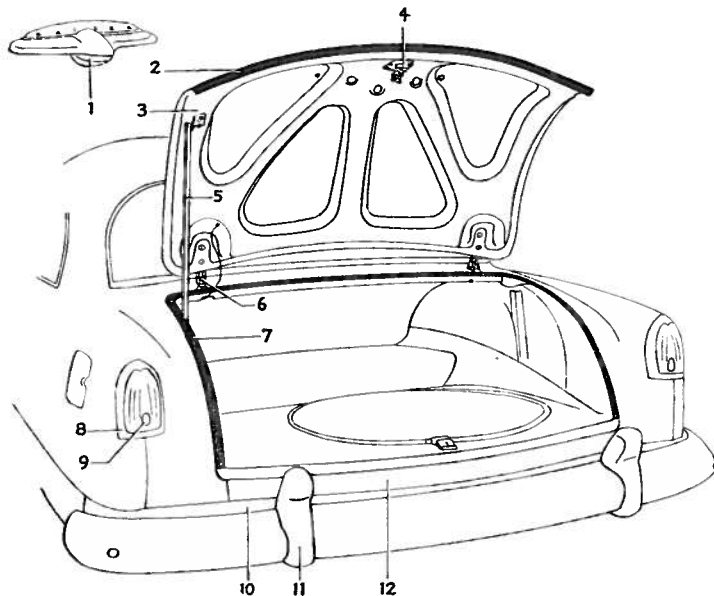
Fig. 7—Rear of Car
