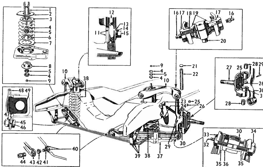
Fig. 10—Front Suspension
