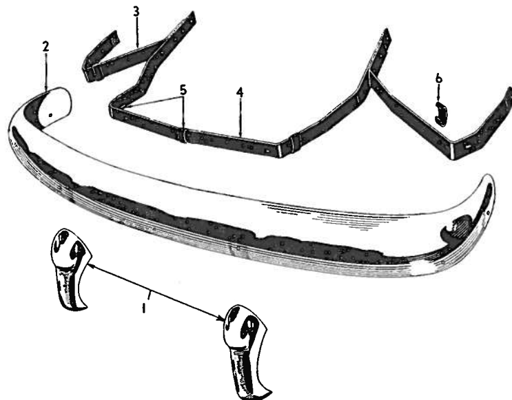
Fig. 2—Front Bumper and Attaching Parts
