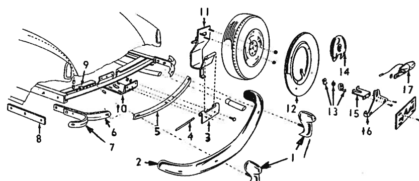
Fig. 8—Spare Wheel Carrier
